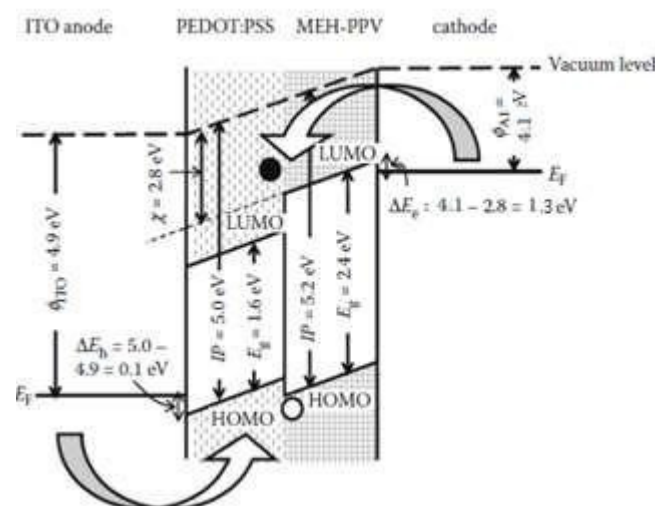
Fig. 2. Energy level diagram of double layer OLED
