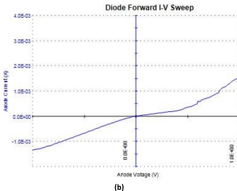
Fig. 4. Measured I-V characteristics of (ITO/ PEDOT: PSS/ MEH-PPV/AL) with PEDOT:PSS thicknesses 50nm and MEH:PPV thicknesses a. 200 nm (1000 rpm), b. 150 nm (2000 rpm)
