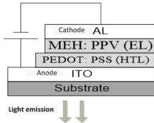
Fig. 1. Double layers OLEDs
