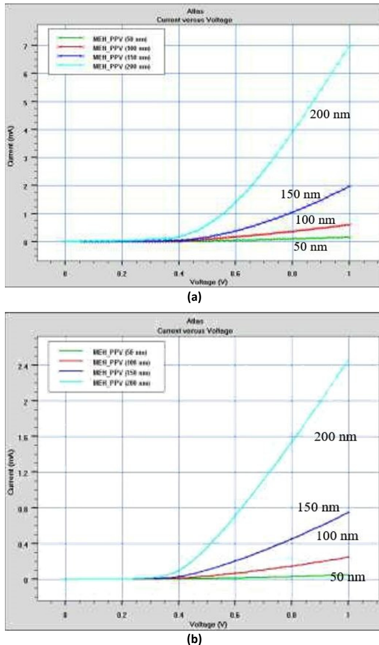
Fig. 3. I-V Characteristics of (ITO/ PEDOT: PSS/ MEH-PPV/AL) with PEDOT:PSS thicknesses a) 50nm, b) 100nm
