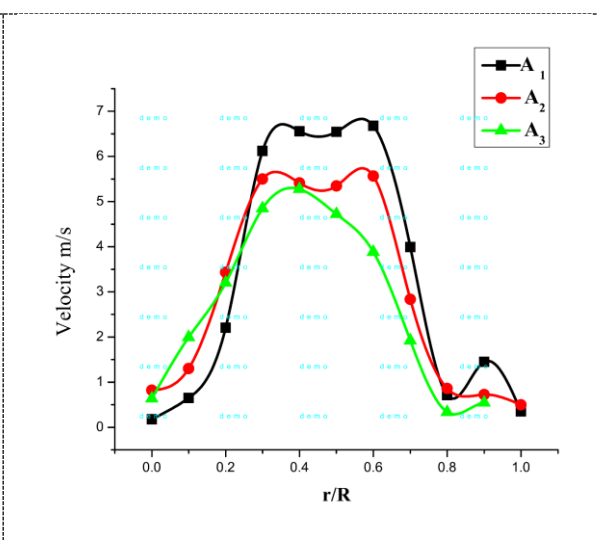
Fig. 12. Significance of momentum Vs. dimensionless distance in the radial direction for 8.31 m/s
