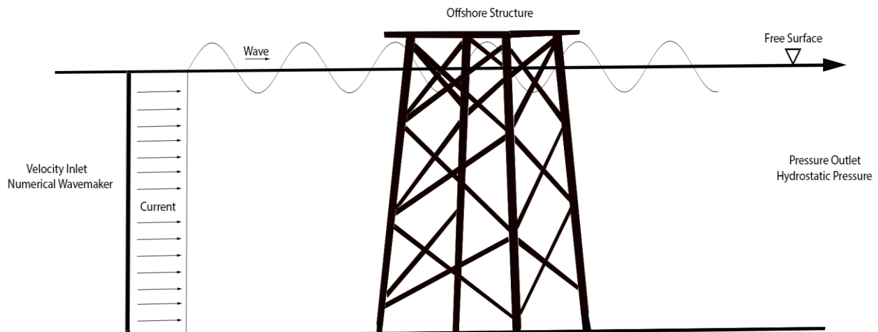
Fig. 1. Sketch of wave and current fields near offshore structure in offshore environment
