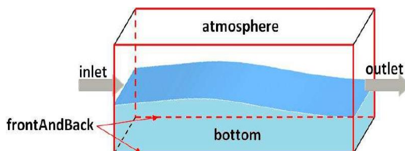
Fig. 2. A numerical wave tank defined with each of its boundary [23]
