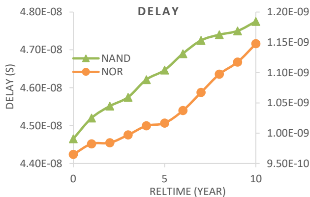
Fig. 11. NAND domino circuit comparison with NOR domino circuit for delay degradation
