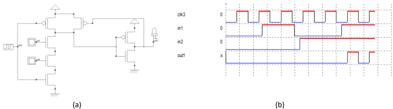
Fig. 5. NAND Domino (a) Schematic diagram (b) Timing diagram
