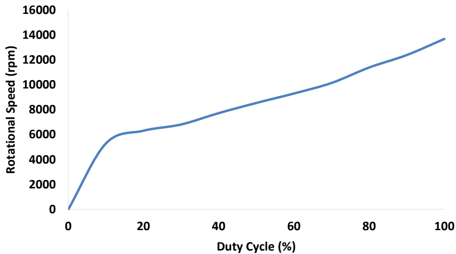
Fig. 10. Valve Duty Cycle vs Rotational speed of turbine
