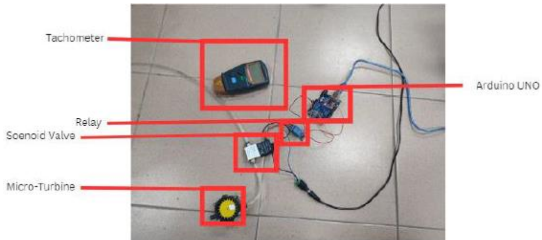
Fig. 5. Test setup for rotational speed measurement of turbine without propeller
