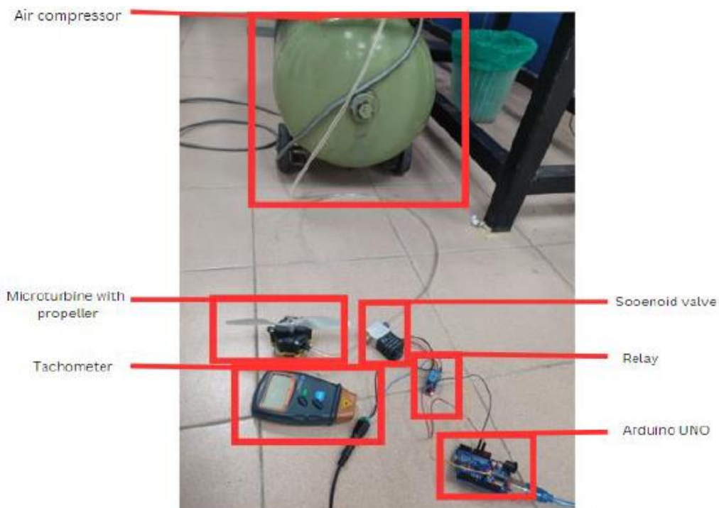
Fig. 6. Test setup for rotational speed measurement of turbine with propeller
