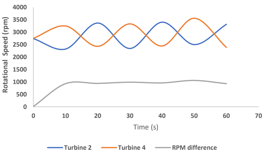
Fig. 12. Turbine Speed vs Time for turbine 2 and 4
