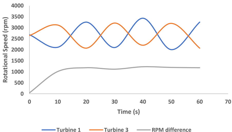
Fig. 11. Turbine Speed vs Time for turbine 1 and 3
