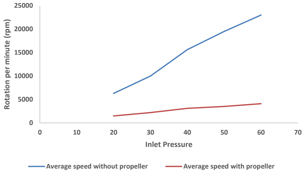
Fig. 9. Inlet air pressure and revolution per minute (rpm) of turbine with and without propeller
