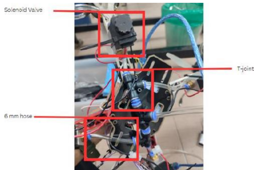
Fig. 4. Hose connection on quadcopter frame
