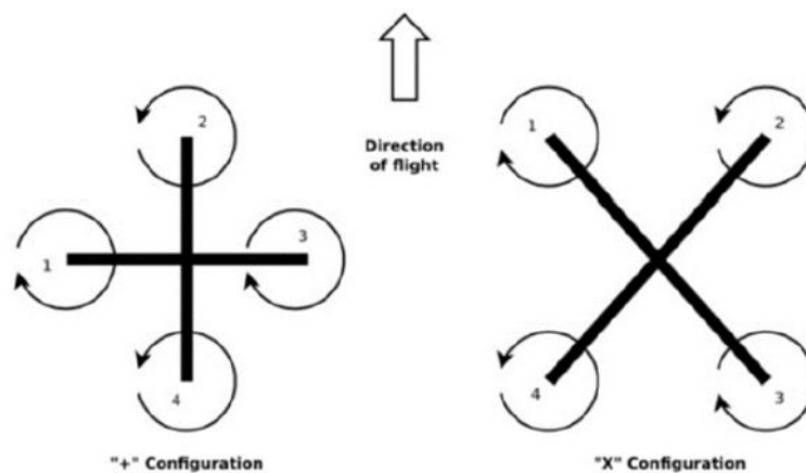
Fig. 1. Two main types of quadcopter configuration [3]
