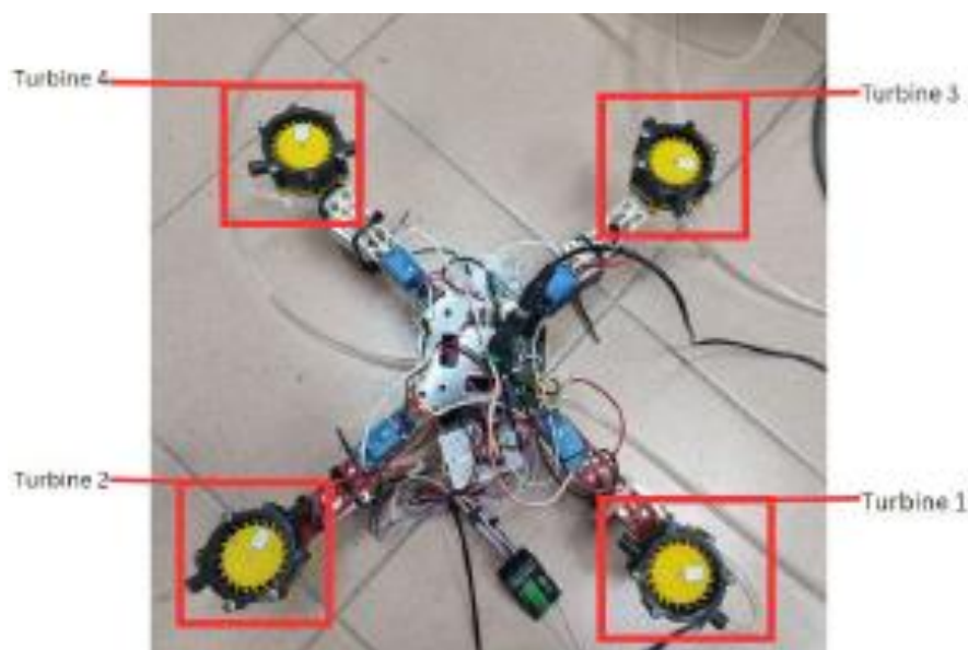
Fig. 8. Setup of turbine drone for testing
