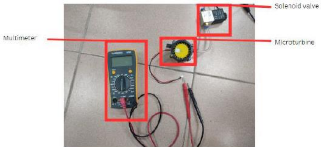
Fig. 7. Setup for voltage reading
