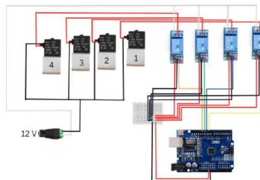
Fig. 3. Control valves system circuit diagram
