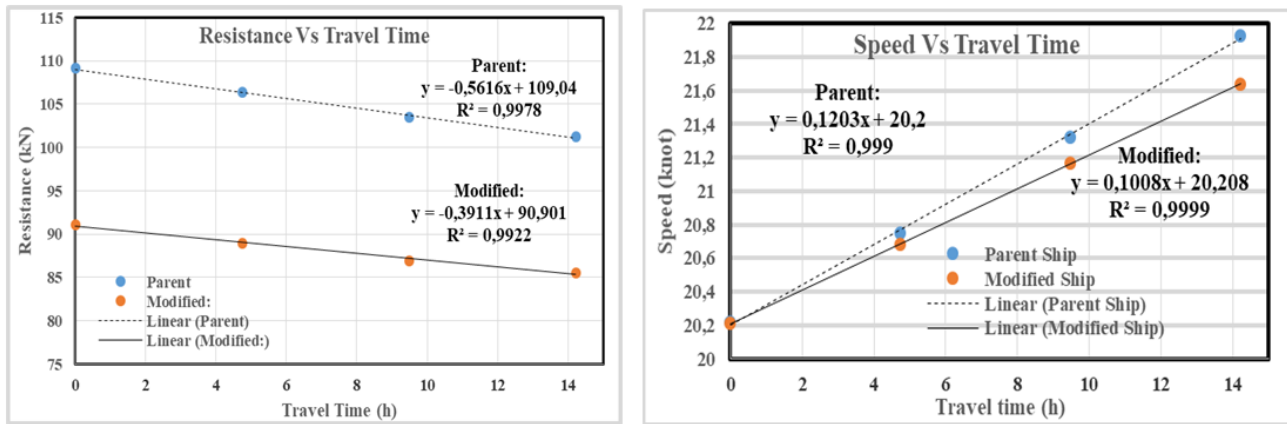
Fig. 5. The changes of Resistance Vs. Travel Time and Speed Vs. Travel Time
