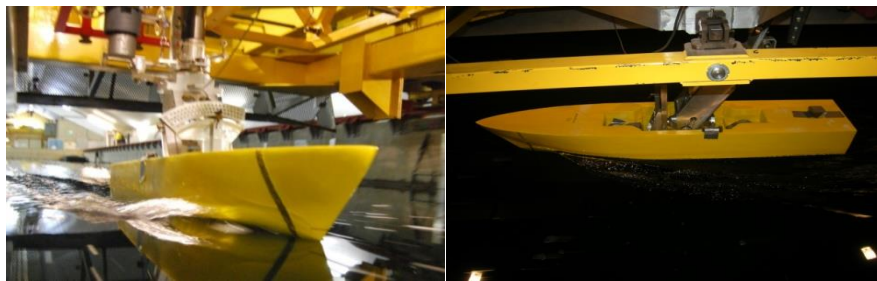
Fig. 3. The ship models are underway
