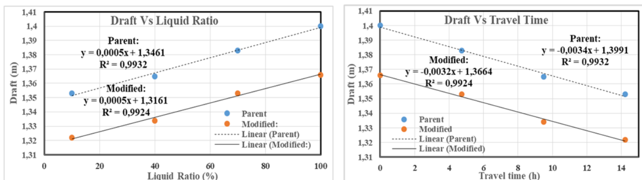
Fig. 4. The Changes of Draft Vs. Liquid Ratio and Draft Vs. Travel Time
