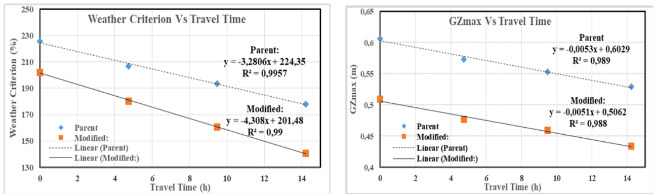
Fig. 6. The Changes of Stability Parameters on Travel Time
