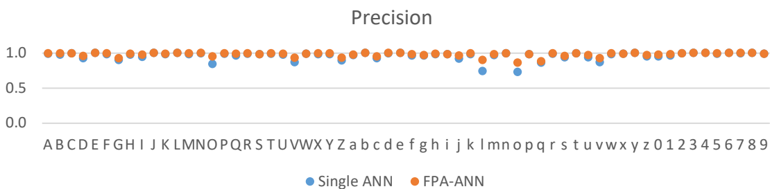
Fig. 4. Comparison of Proposed FPA-ANN and Single ANN in term of Precision
