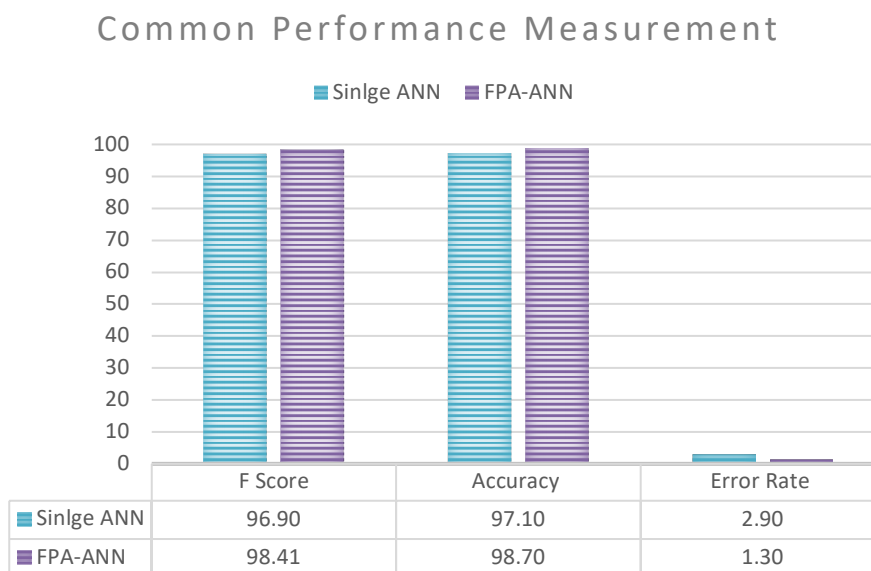
Fig. 7. Comparison of Proposed FPA-ANN and Single ANN in term of F-Score, Accuracy and Error Rate
