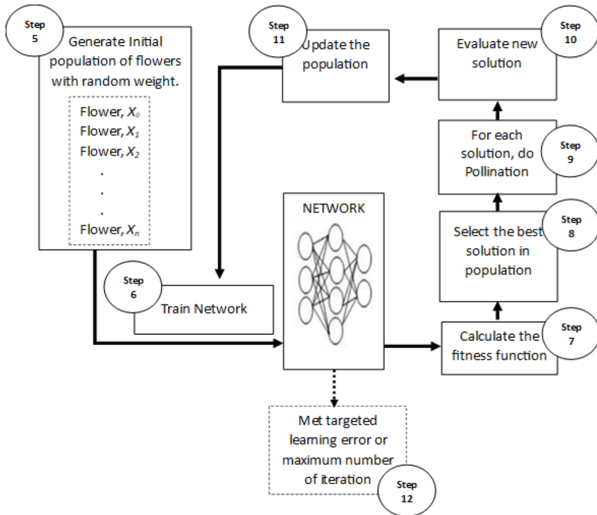
Fig. 3. Illustration of Flower Pollination Algorithm Optimization in ANN Network Training
