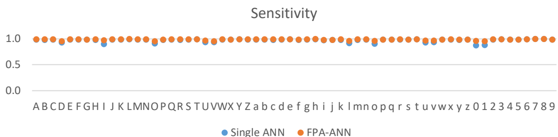
Fig. 5. Comparison of Proposed FPA-ANN and Single ANN in term of Sensitivity
