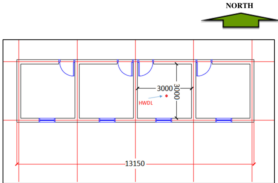
Fig. 3. Floor Plan of the Non-Courtyard House (Case-study 1)
