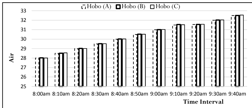
Fig. 8. Air Temperature of the three HWDL
