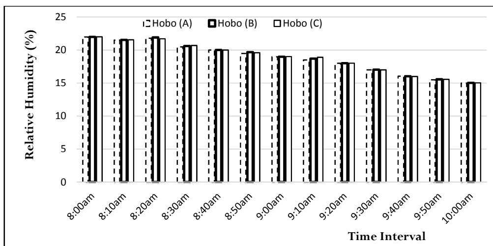
Fig. 9. Relative Humidity of the three HWDL
