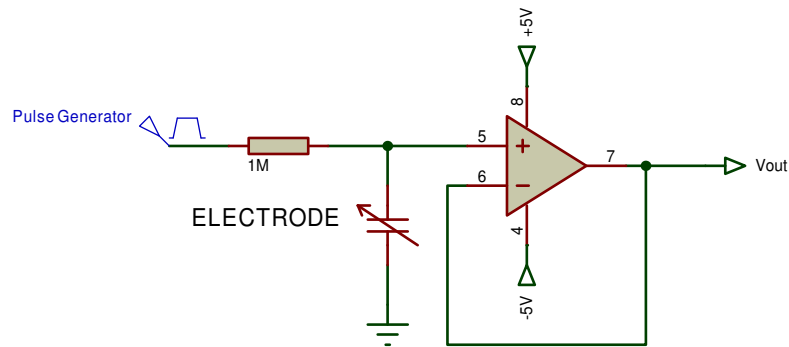
Fig. 5. Charge transfer capacitive sensor
