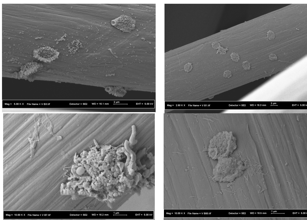
Fig. 3.4. FESEM image of bacteria attachment to graphite felt electrode
