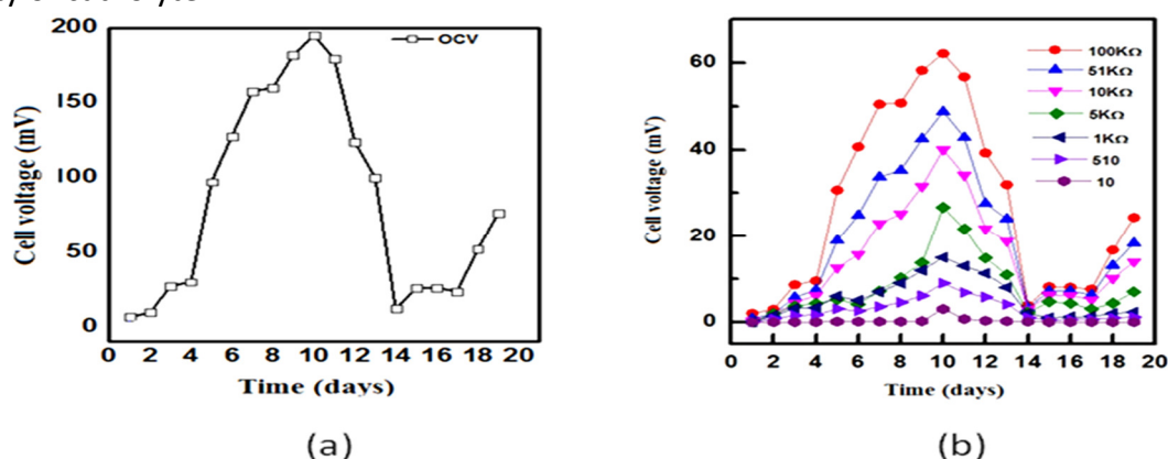
Fig. 3.1. Plant microbial fuel a: Open circuit cell voltage (OCV) and b: Close circuit voltage (CCV). Consequently, The arrow indicates 2 mL 1 M phosphate buffer addition to the cathode chamber.
