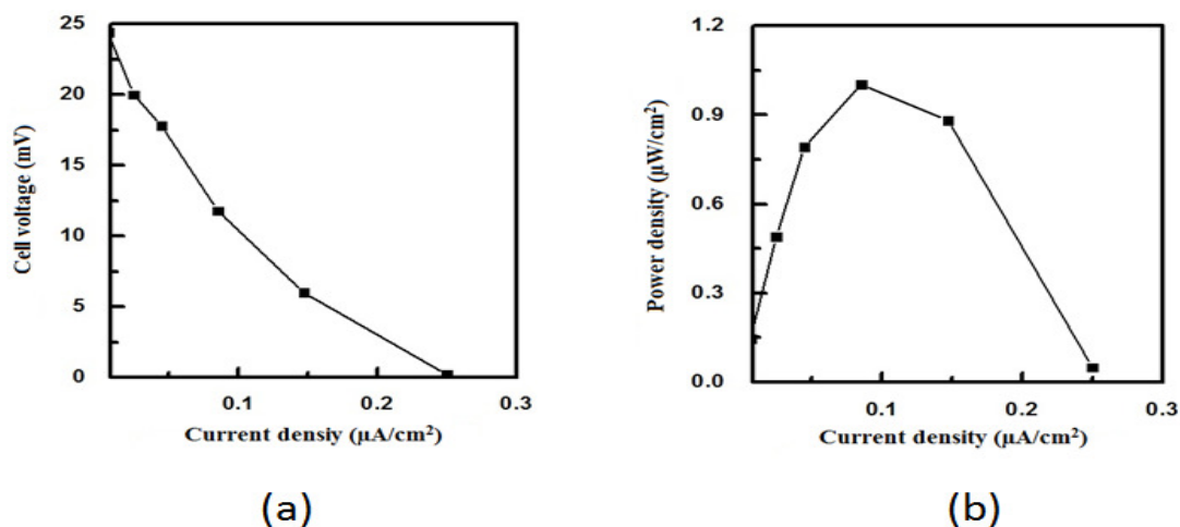
Fig. 3.2. (a) Polarization curve with cell voltage, (b) with Plant MFC.
