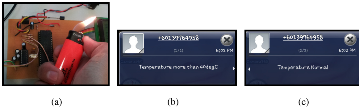
Figure 6: (a) The method to make the temperature sensor activate the PIC 16F877A microcontroller (b) Alarm message when the temperature more than 40°C (c) The messages that show the temperature is in normal condition
