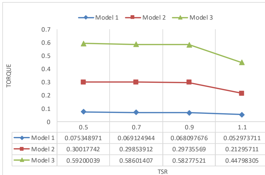
Fig. 1. Torque against the tip-speed ratio for all models
