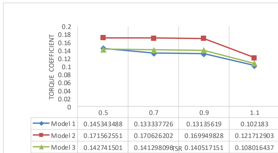
Fig. 2. Torque coefficient against TSR comparison for all models
