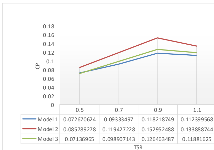
Fig. 4. Comparison of C_p against TSR for 3 Model
