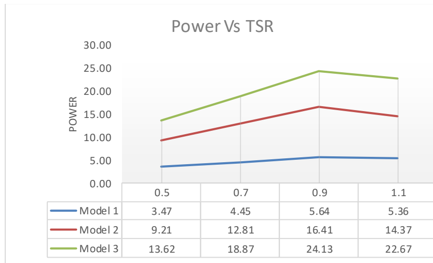
Fig. 3. Power against TSR comparison for 3 models
