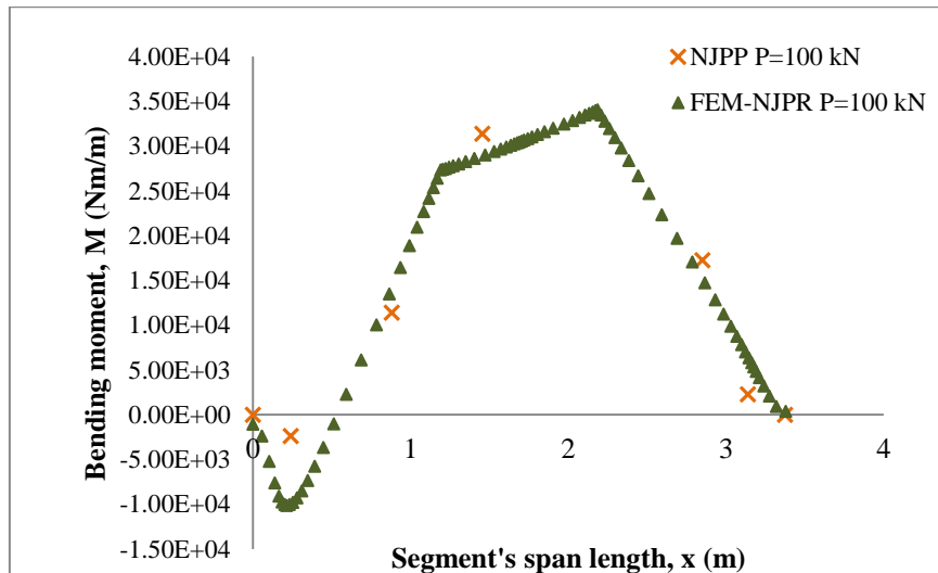
Fig. 8. Bending moment for pin-roller support condition (NJPR) with numerical modelling result (FEM-NJPR) of single segment
