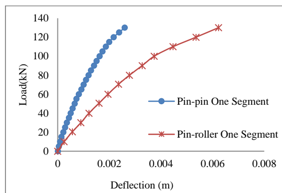
Fig. 5. Load vs deflection at mid span of segment
