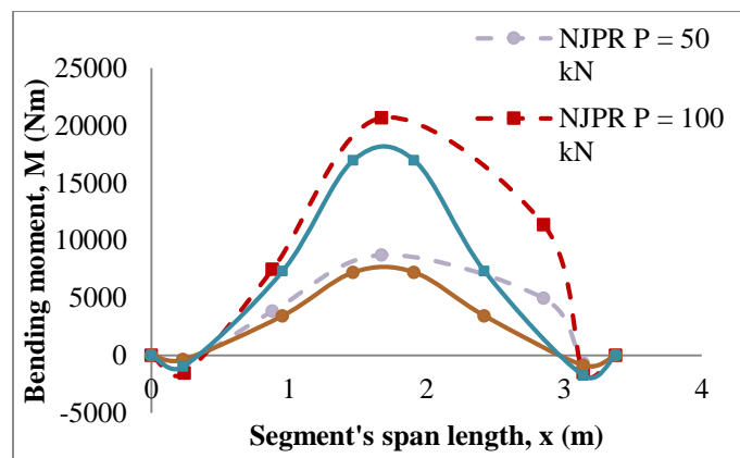
Fig. 6. Bending moment for non-jointed pin-roller test (NJPR) and non-jointed pin-pin test (NJPP) of single segment
