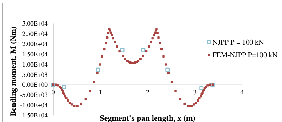
Fig. 7. Bending moment for pin-pin support condition (NJPP) with numerical modelling result (FEM-NJPP) of single segment
