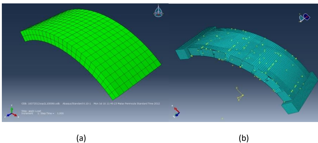
Fig. 1. Segment lining in mesh (a) Single segment (b) Dual jointed segment with pairs of pedestal
