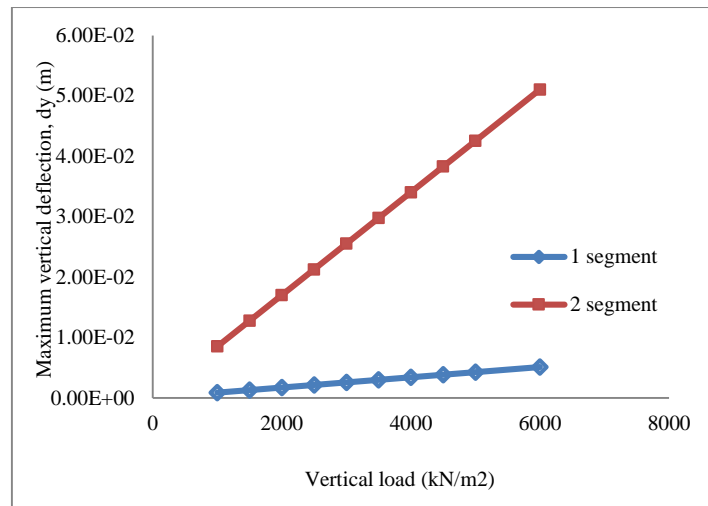
Fig. 2. Load - deflection curves of one segment and dual jointed segment
